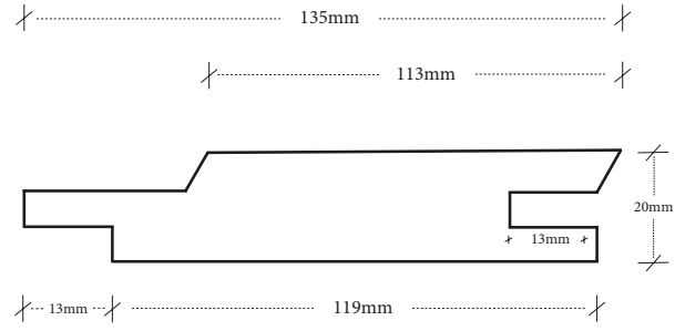
GT 15 20x135 (119mm)
