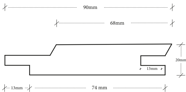
GT 14 20x90 (74mm)
