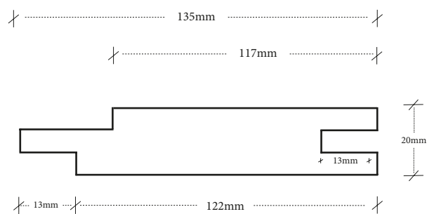
GT 13 20x135 (122mm)
